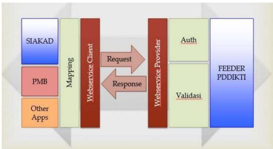
Gambar 2.1 Skema Interoperabilitas Neo Feeder
